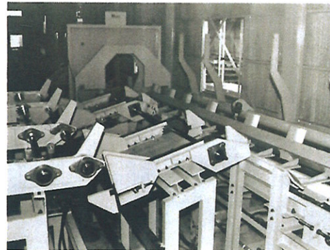
▲原木自動計測機 Automatic Scanner & Infeed Equipment
