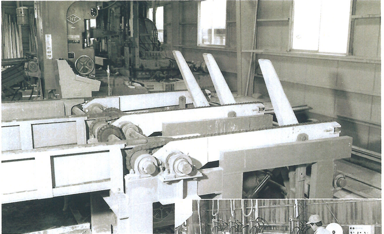
▲原木搬入盤台 Chain Live Deck Chain Loader Deck Flipper
