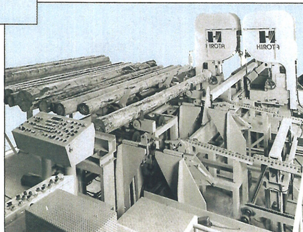
▲ツインバンド用搬送装置 Conveying Equipment for Twin Band Saw Mill
